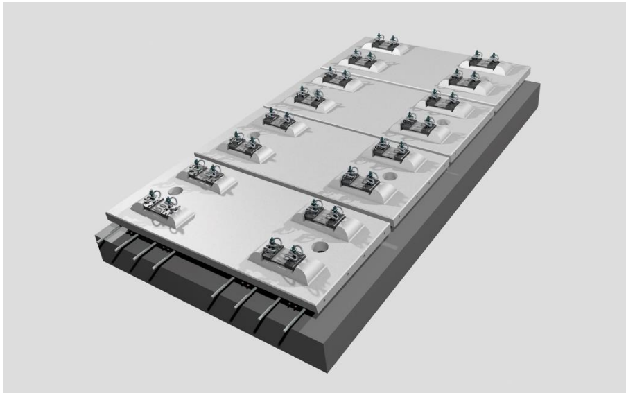
Caption 1: Animation of RAILONE ROCS slab track system
